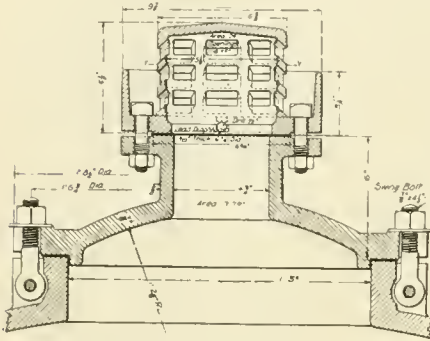
SAFETY VALVE FOR TANK CARS.
